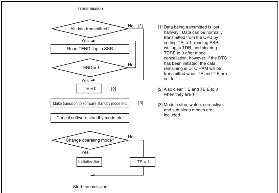
Figure 13.34 Sample Flowchart for Mode Transition during Transmission
