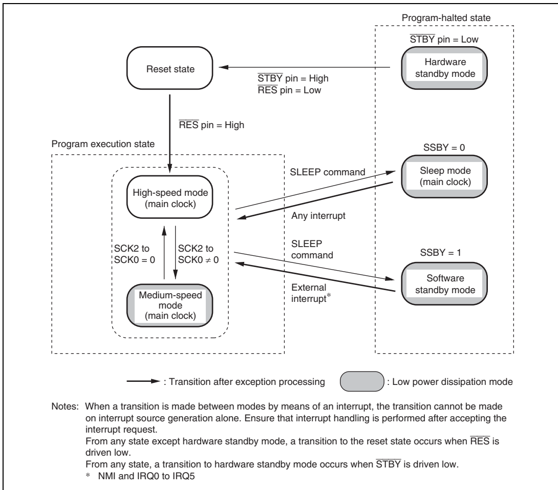
Figure 18.1 Mode Transition Diagram
