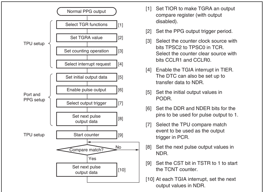
Figure 11.4 Setup Procedure for Normal Pulse Output (Example)
