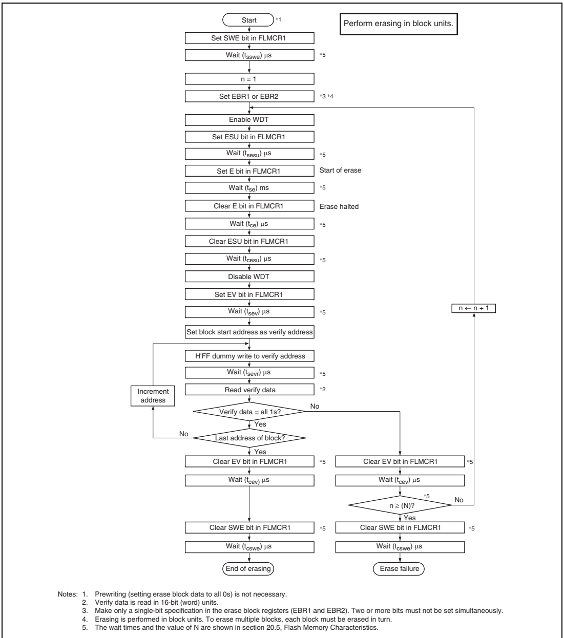
Figure 16.10 Erase/Erase-Verify Flowchart
