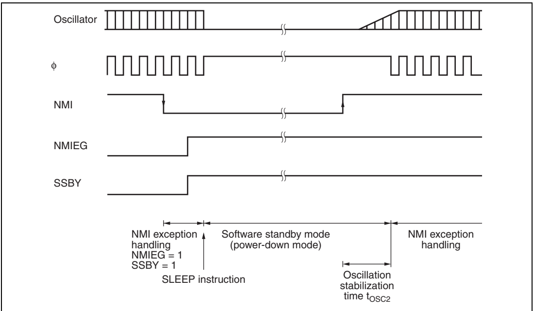
Figure 18.3 Software Standby Mode Application Example
