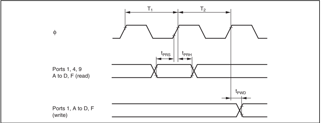
Figure 20.6 I/O Port Input/Output Timing
