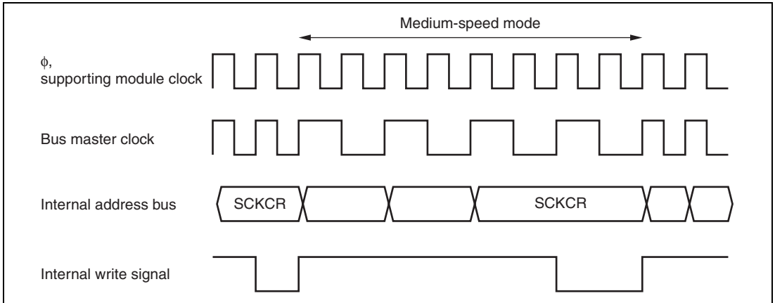
Figure 18.2 Medium-Speed Mode Transition and Clearance Timing
